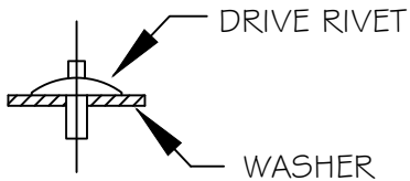
SIGN DRIVE RIVET DETAIL FOR MOUNTING SIGN
